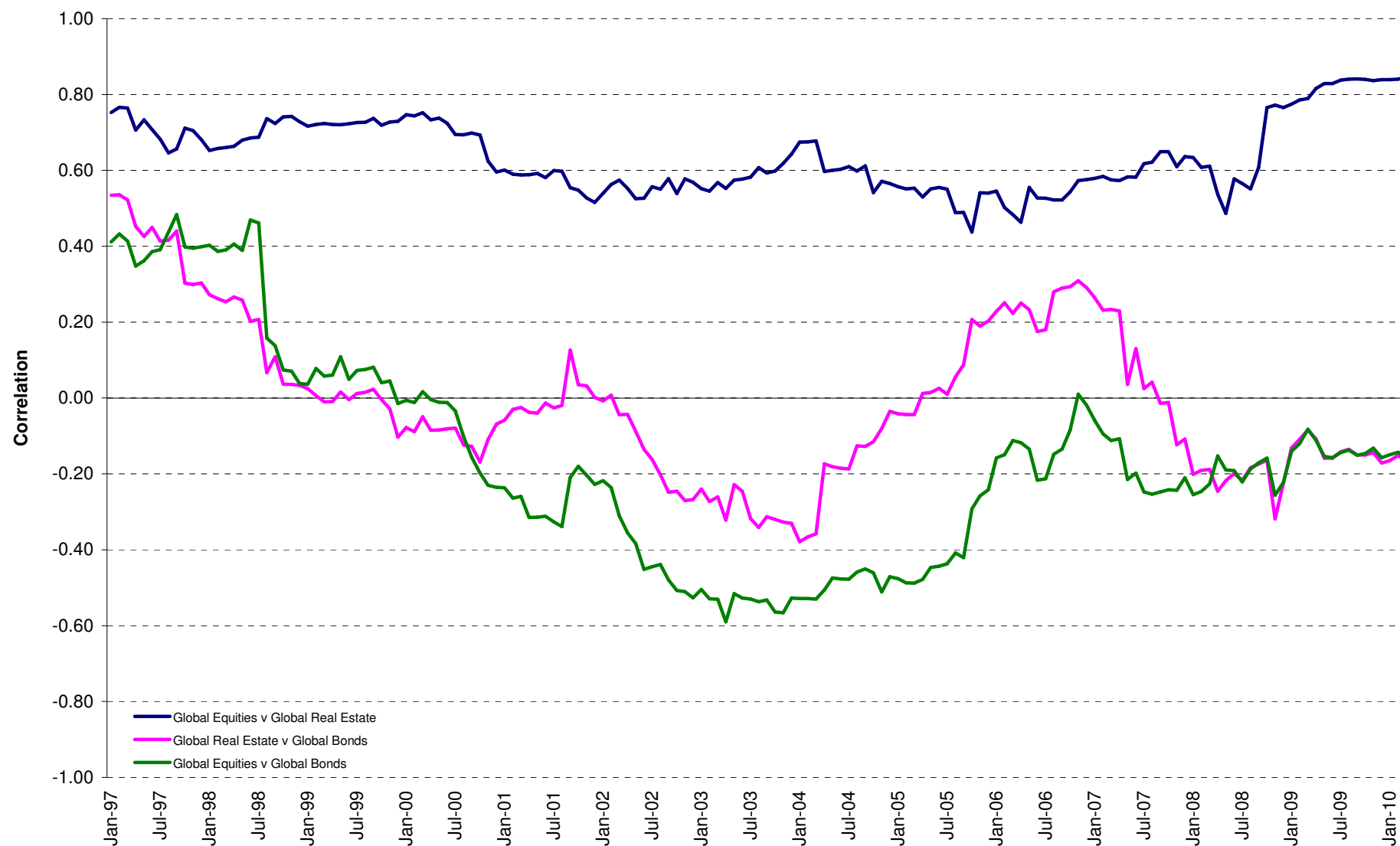
Graph 34: Developed Real Estate, Equities & Bonds 36 Months Asset Class Correlations (Local) 1997 to Date
