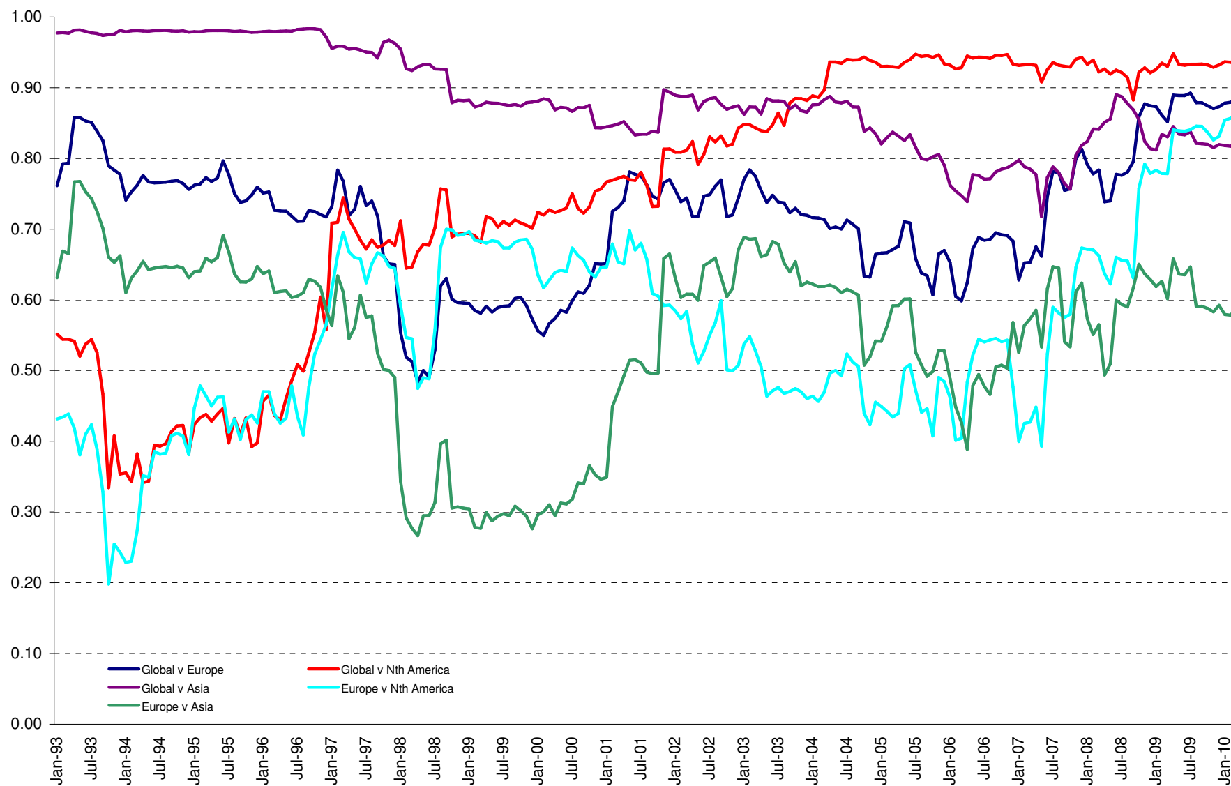
Graph 37: Global Developed & Developed Regional 36 Months Correlations (EUR) 1993 to Date
