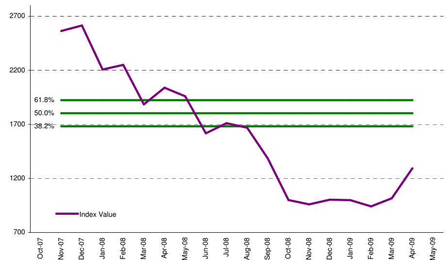
Graph 88: 1Y Retracement Levels - Emerging Markets
