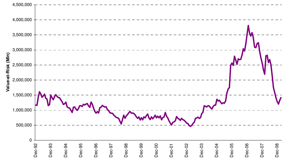
Graph 122: Equally Weighted Value-at-Risk - Japan
